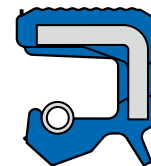
Design BA..SL conforming to DIN / ISO Design AS Grooved OD
